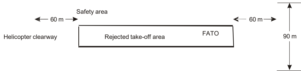
Figure A-1. Safety area for instrument FATO
